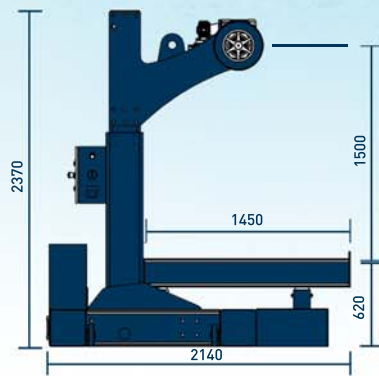
CLOSED POSITION
